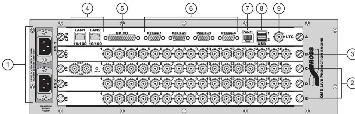
Synergy Q/MD Frame — Rear View
