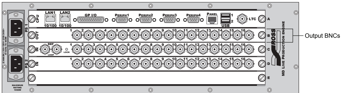
Synergy Q/MD Frame - Rear Output Section
