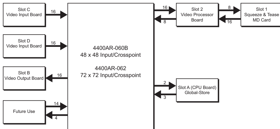
Video Flow Through 48 x 48 Crosspoint Matrix
