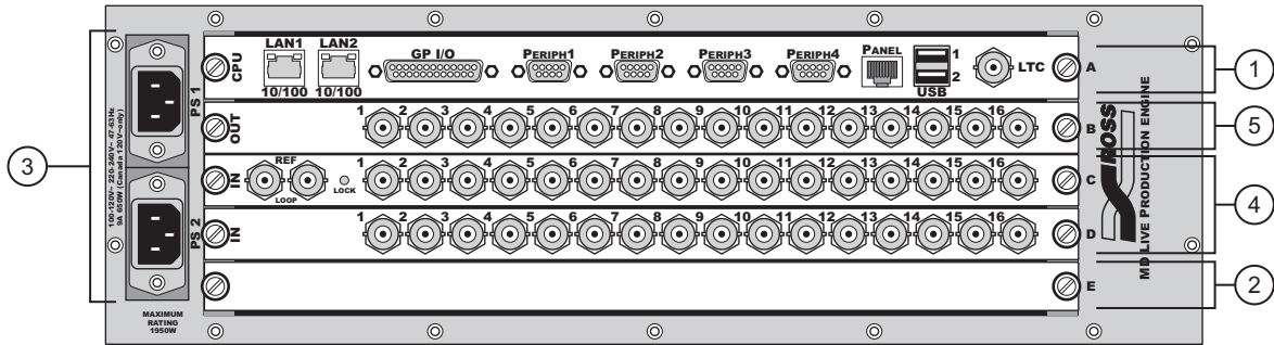
Synergy Q/MD Frame — Rear View
