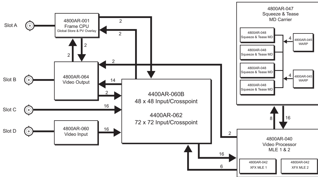
Synergy Q/MD Block Diagram - 48 x 48 Crosspoint
