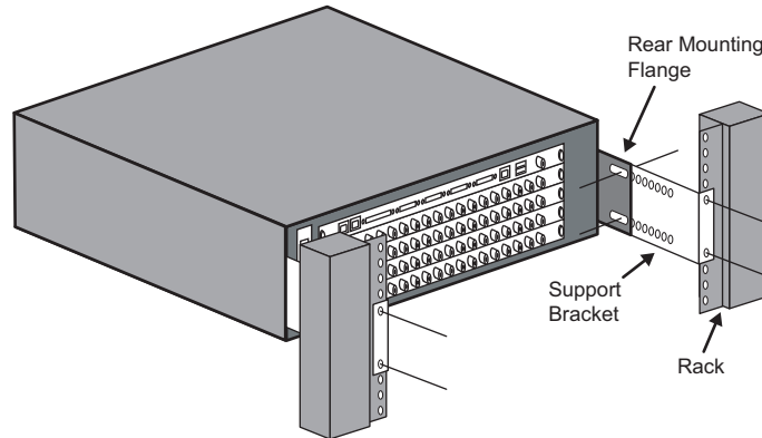
Rear of Synergy Q/MD Frame with Support Brackets Installed
