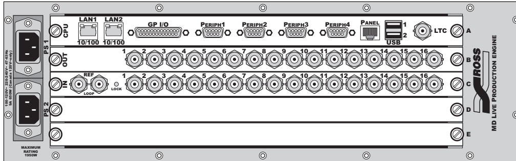
Synergy Q/MD Frame — Default Board Locations
