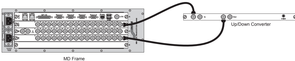
Synergy Q/MD Frame - Up/Down Converter Conversion Loop Output Section
