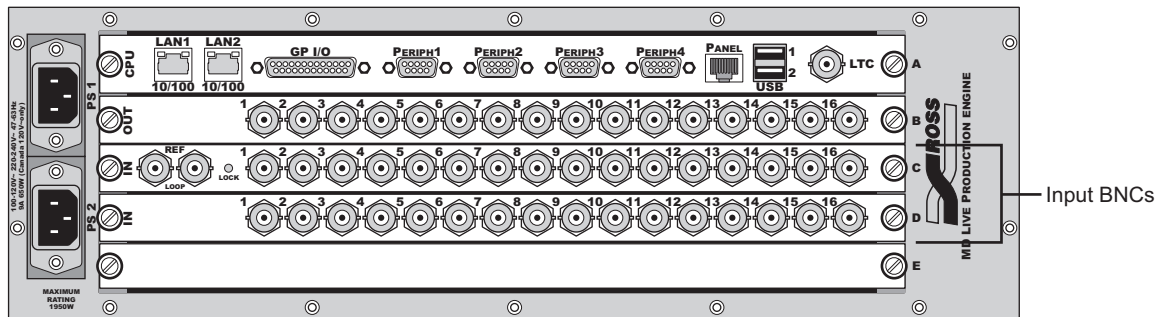
Synergy MD Chassis — Rear Input Section
