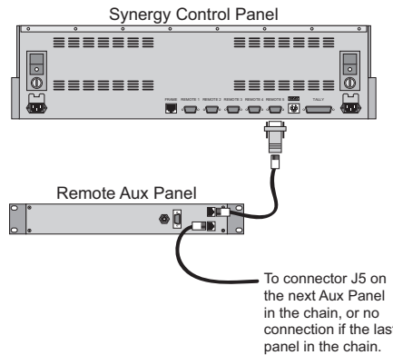
Remote Aux Panel Interconnection — Synergy 1 Control Panel
