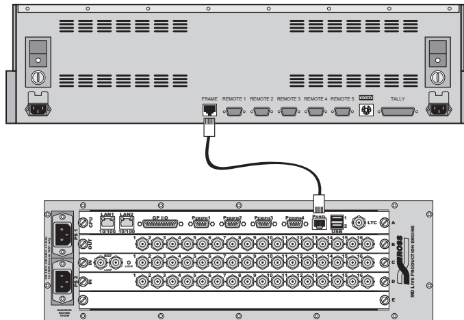
Synergy Q/MD Frame to Synergy 1 Control Panel Interconnection
