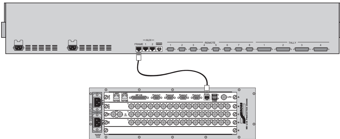
Synergy Q/MD Frame to Synergy 2.5 Control Panel Interconnection
