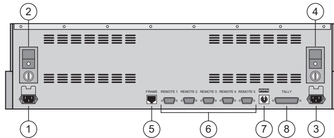
Synergy 1 Control Panel — Rear View, Connector Section
