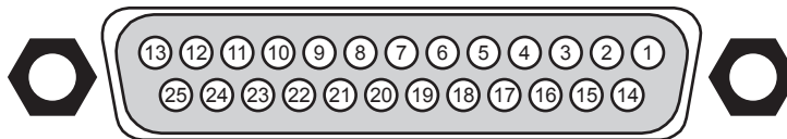
Synergy 1 — Tally Port Pinout
