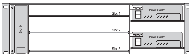
Figure 6.1 Board Slots in the Front of the Q/MD Frame
