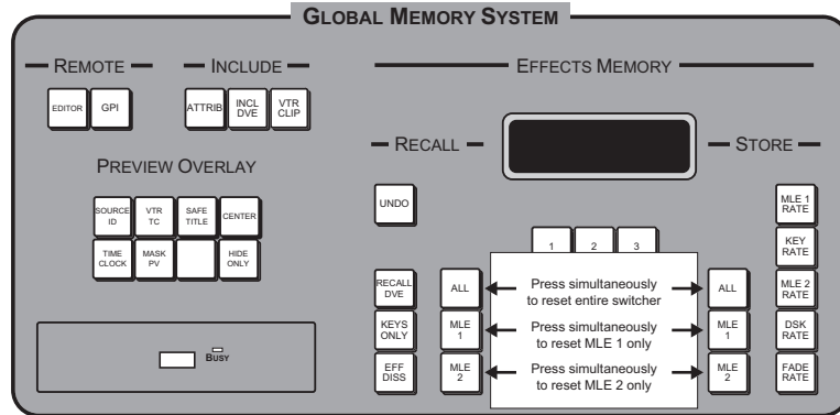
Synergy 2 — Global Memory System Group Reset Function
