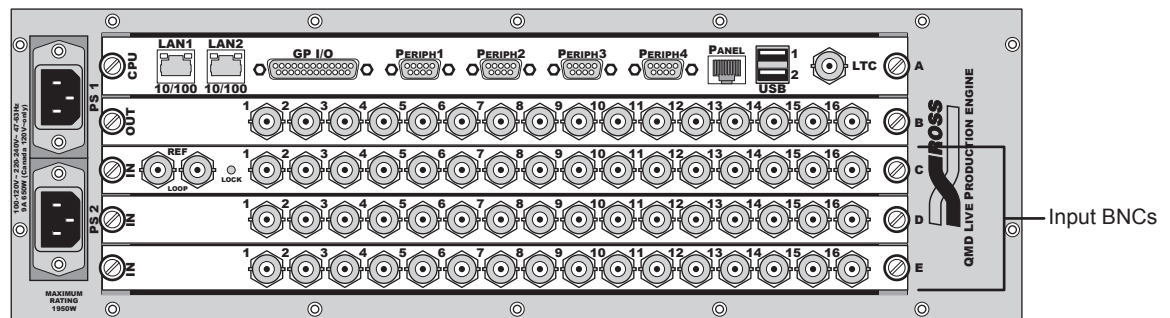
Synergy Q/MD Chassis — Rear Input Section
