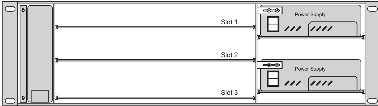
Board Slots in the Front of the Q/MD Frame
