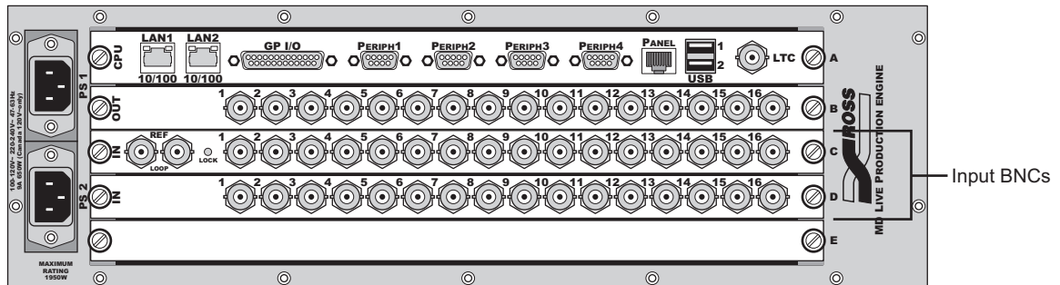
Synergy Q/MD Frame - Rear Input Section
