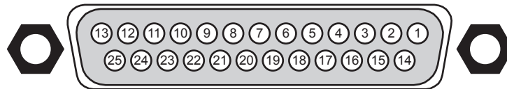
Tally Port Pinout
